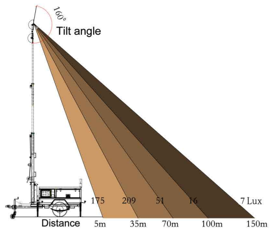
LED light (4x400W)
