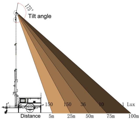
Metal halide (4x1000W)
